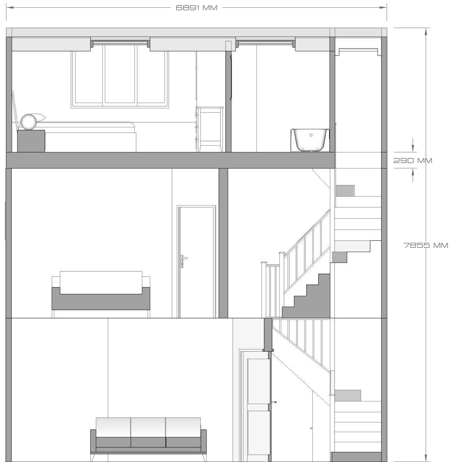
SECTION YY, WHOLE BUILDING
