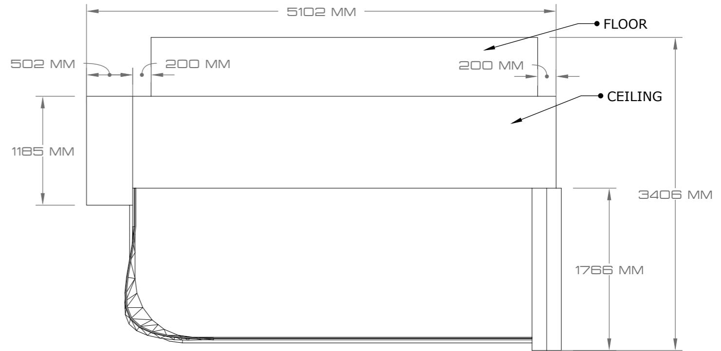
SHOP TOP B/W
