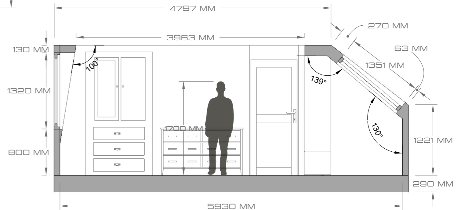
SECTION EE, 2ND FL
