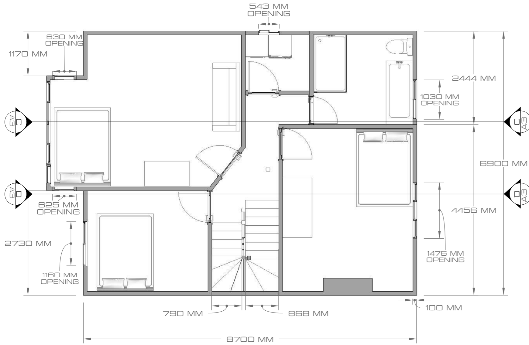
TOP VIEW THROUGH WINDOWS, 1ST FL
