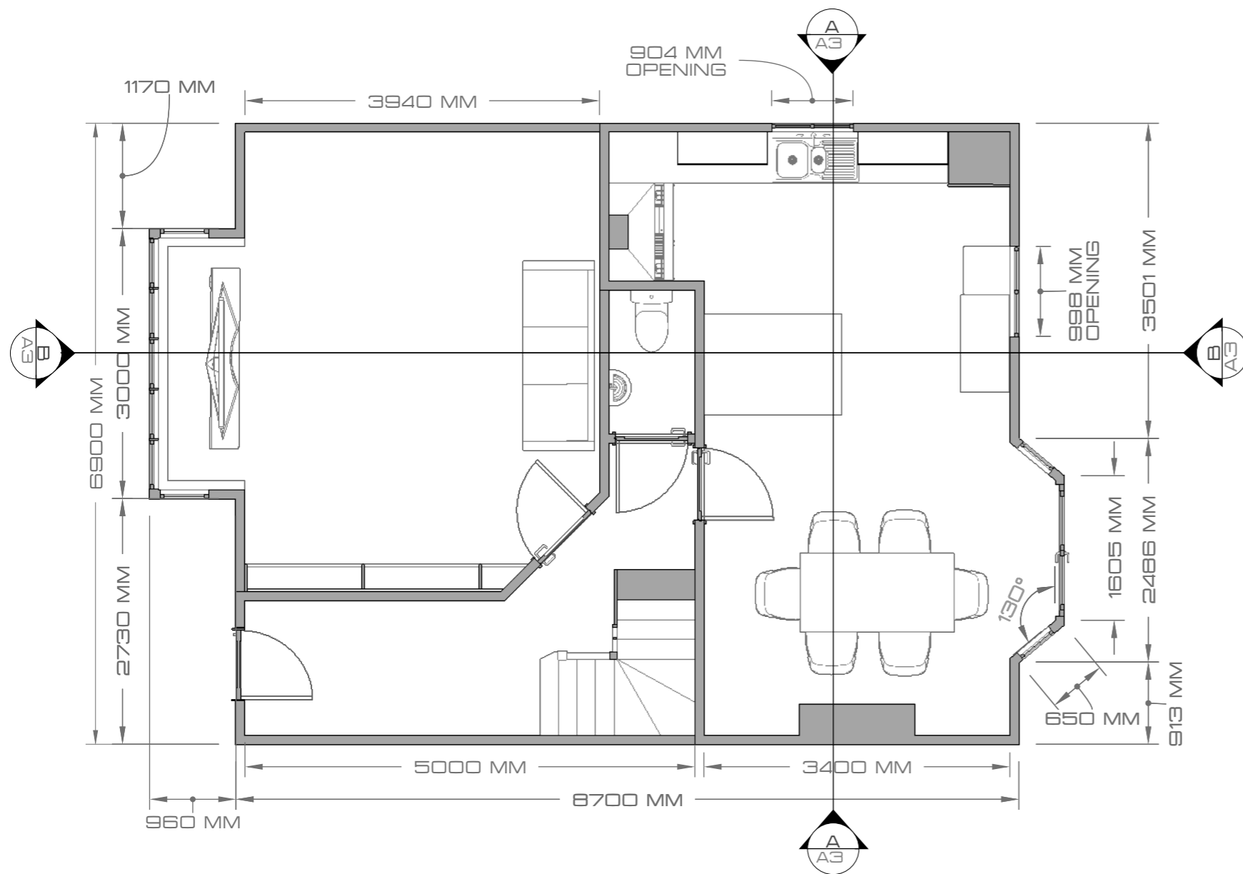
TOP VIEW THROUGH WINDOWS, GROUND FL
