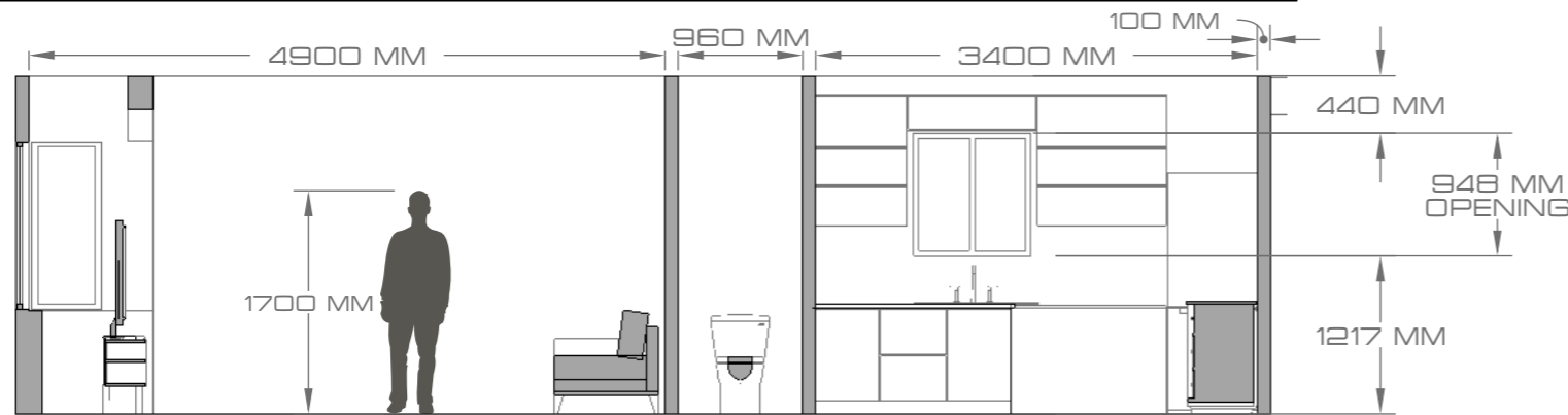
SECTION AA, GROUND FL
