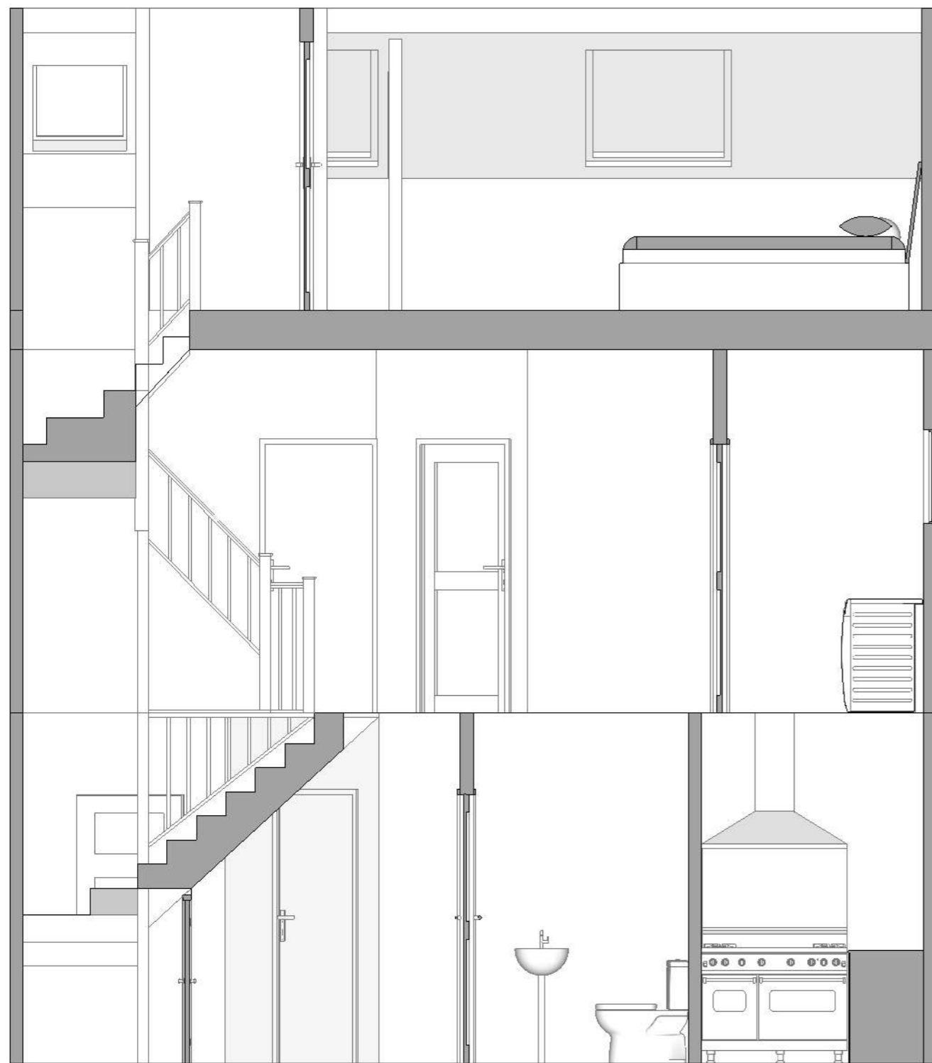
SECTION XX, WHOLE BUILDING
