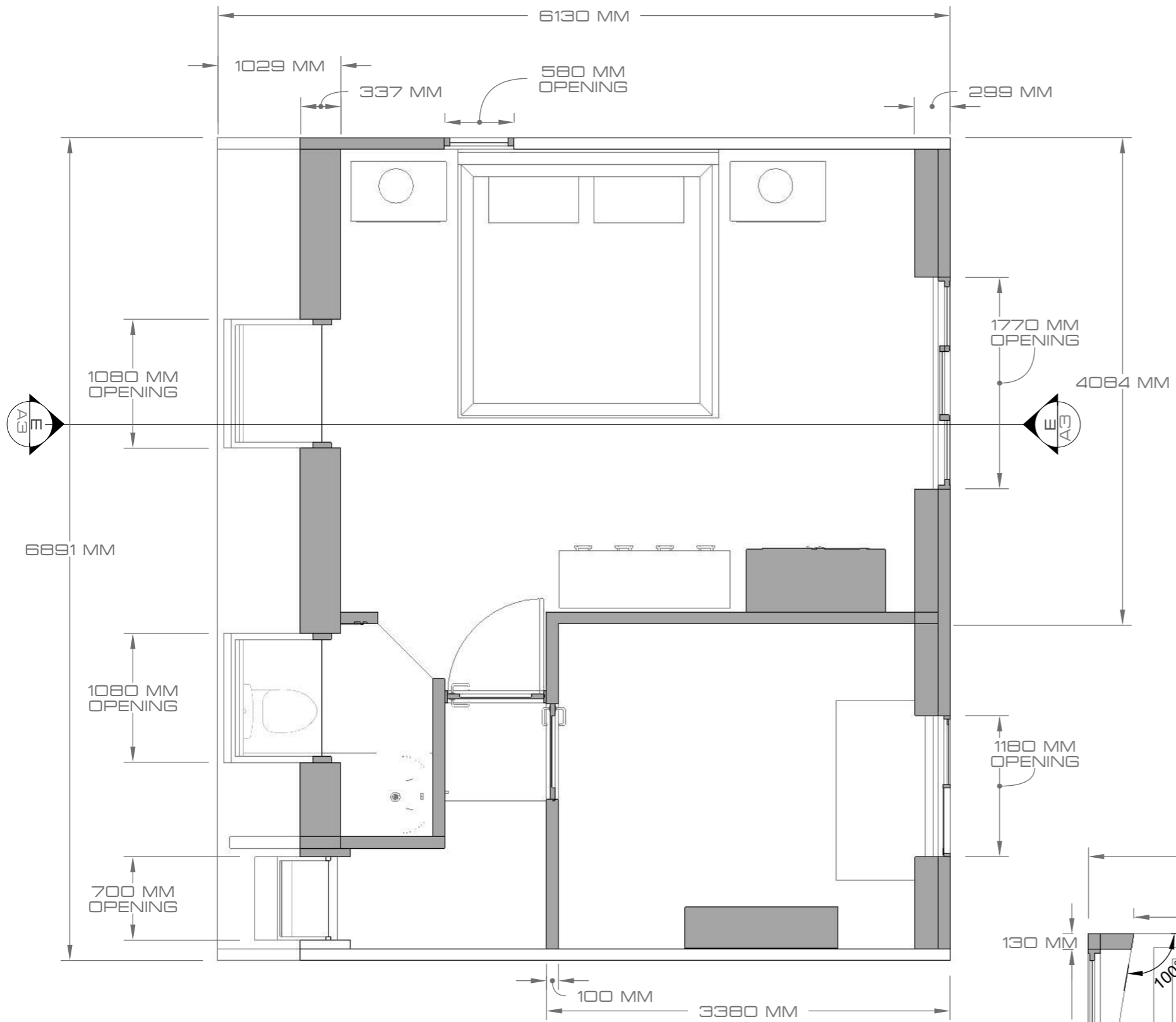
TOP VIEW THROUGH WINDOWS, 2ND FL
