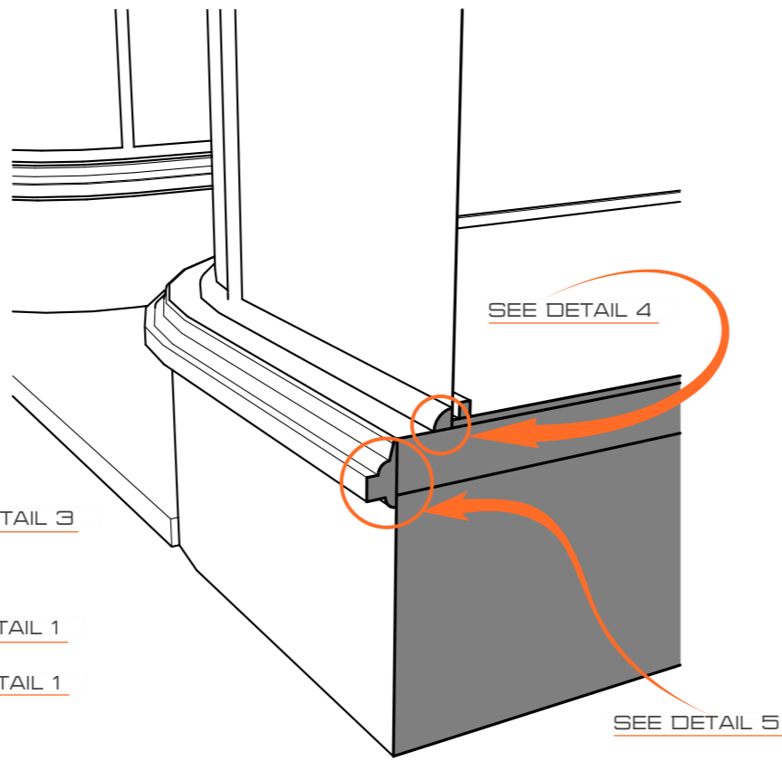
LOWER MOLDINGS VIEW
