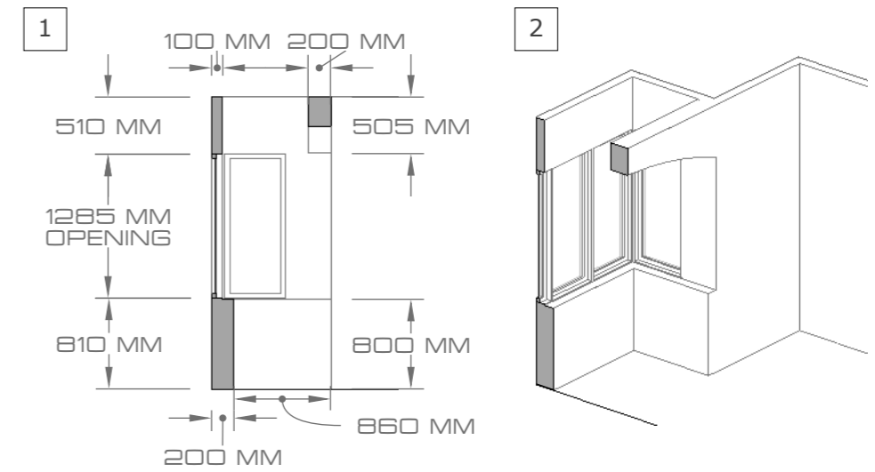
OVERALL VIEW, GROUND FL
