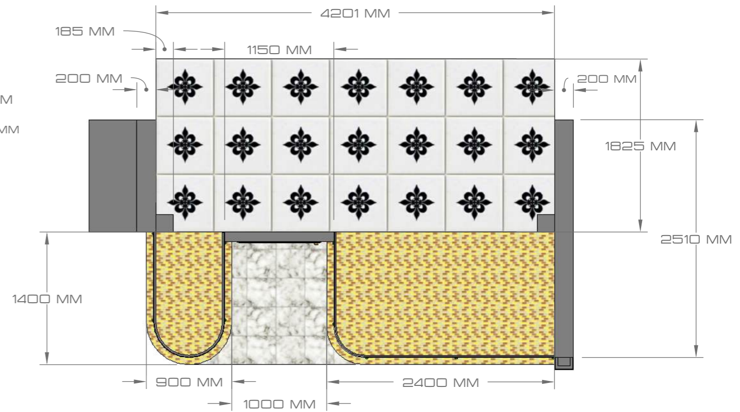
SECTION JJ (NO MOLDINGS)
