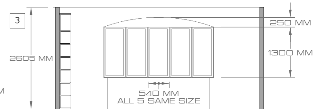
WINDOW DETAIL, GROUND FL
