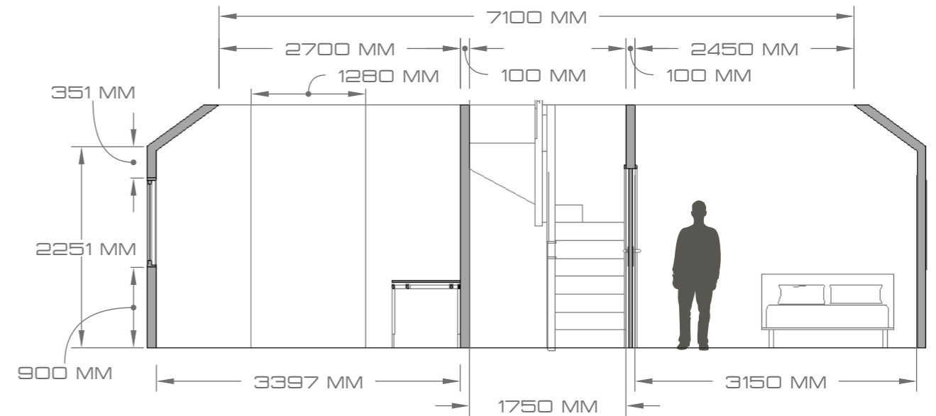
SECTION DD, 1ST FL
