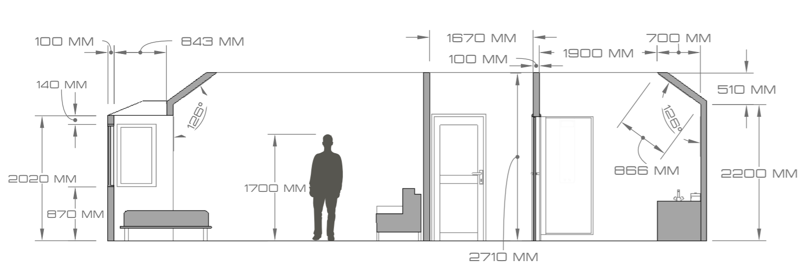
SECTION CC, 1ST FL
