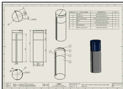
Design Project: Sustainable Mug CAD (SolidWorks) / Technical Drawing
