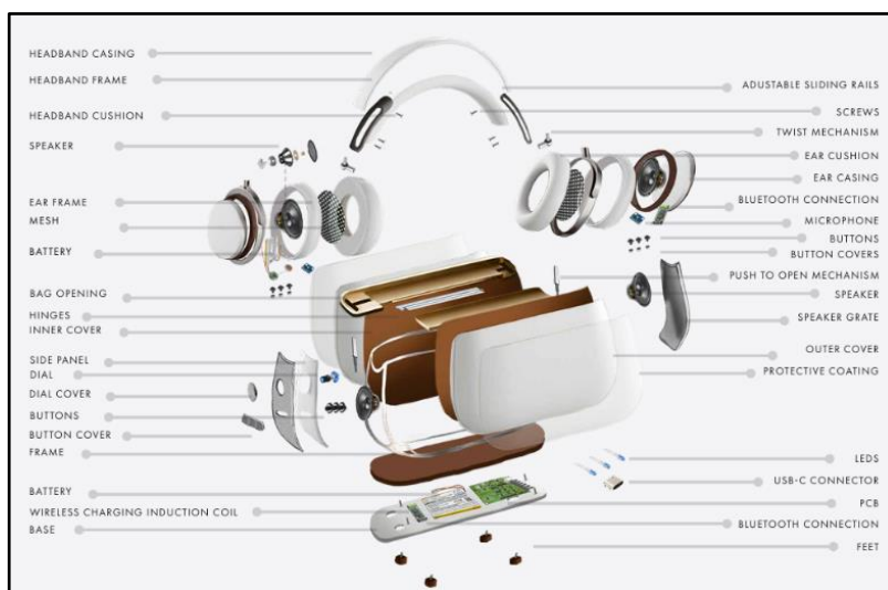
Design Project: Exploded Drawing Adobe Photoshop/InDesign
